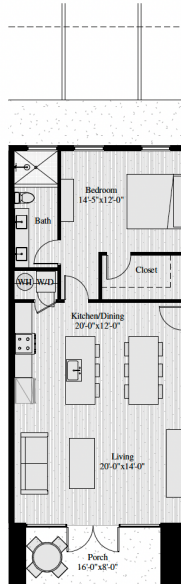
Type B - 1 Bed/1 Bath Units 102 & 103 - Level 1 only Total square footage heated/cooled - 937 SF Porch - 118 SF
