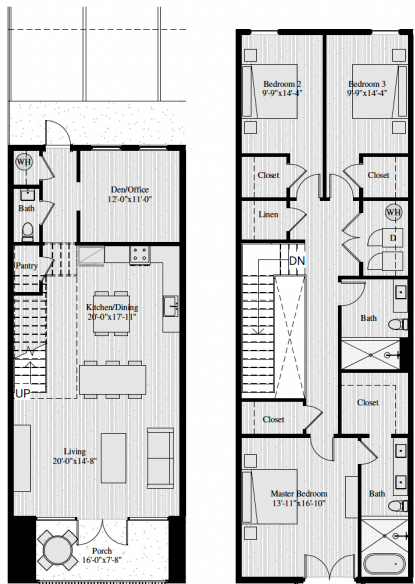
Type A - Two-Story Rowhouse - 3 Bed/2.5 Bath Units 101 & 104 Main Level - 952 SF Second Level - 1,400 SF Total square footage heated/cooled - 2,352 SF Level 1 Porch - 118 SF
